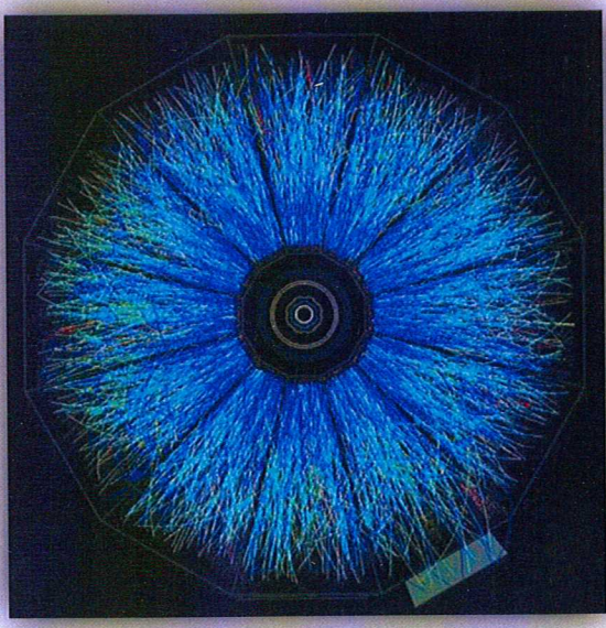
Exploded gold ions
