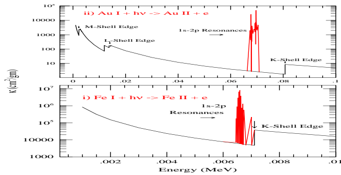
Figure 8. High peak resonances below the K-shell ionization threshold of i) iron and ii) gold arising from K_{\alpha} ( 1s-2p ) transitions. The resonances correspond to all allowed K_{\alpha} transitions of the Ne- to He-like ions as the element goes through multiple ionization stages at a resonant energy (Pradhan et al 2009).
