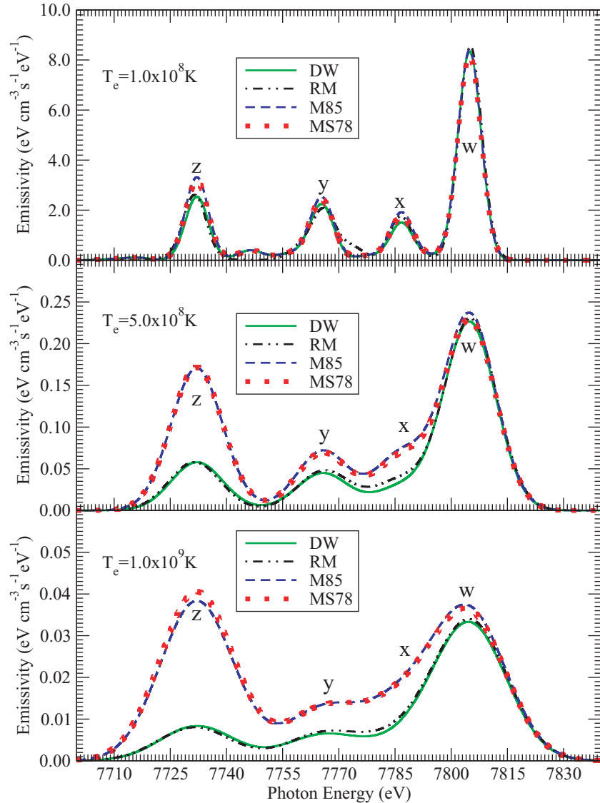
Figure 2. Emission spectra of a low-density ( N_e = 10^{10} \text{cm}^{-3} ) Ni plasma at three different temperatures in the high-temperature range where the G ratio from the models is in poor agreement. Spectra from the DW, M85 and MS78 models have all been redshifted by 9 eV to facilitate an easier comparison.
