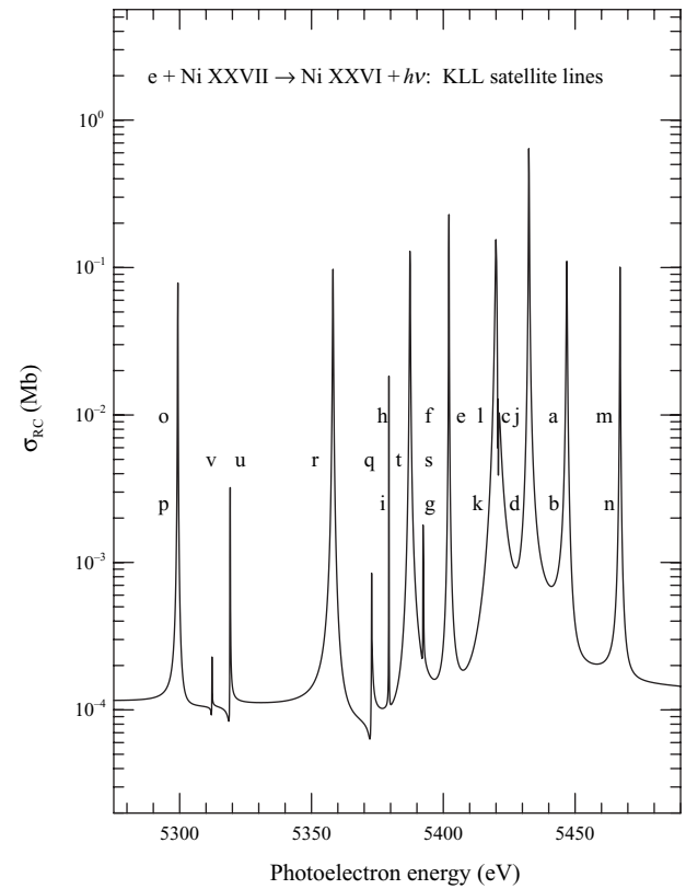
Figure 2. Theoretical profiles of the 22 DES lines of the K\alpha complex seen in unified recombination cross sections of Ni XXVII, as in figure 1.
