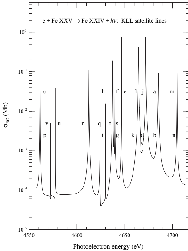
Figure 1. Theoretical profiles of the 22 DES lines of the K\alpha complex seen in unified recombination cross sections of Fe XXV. The interference effects in the ab initio results manifest themselves in the natural overlap of line profiles as described in the text.
