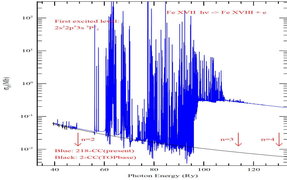
Figure 6. \sigma_{PI} of the first single valence electron excited level of 2s^2 2p^5 3s(^3P^o_2) of Fe XVII, demonstrating impact of the n = 3 complex of resonances forming strong resonance features that are several orders of magnitude higher than those due to the n = 2 complex and background enhancement near the n = 3 threshold; however, beyond the n = 3 resonances are very weak.
