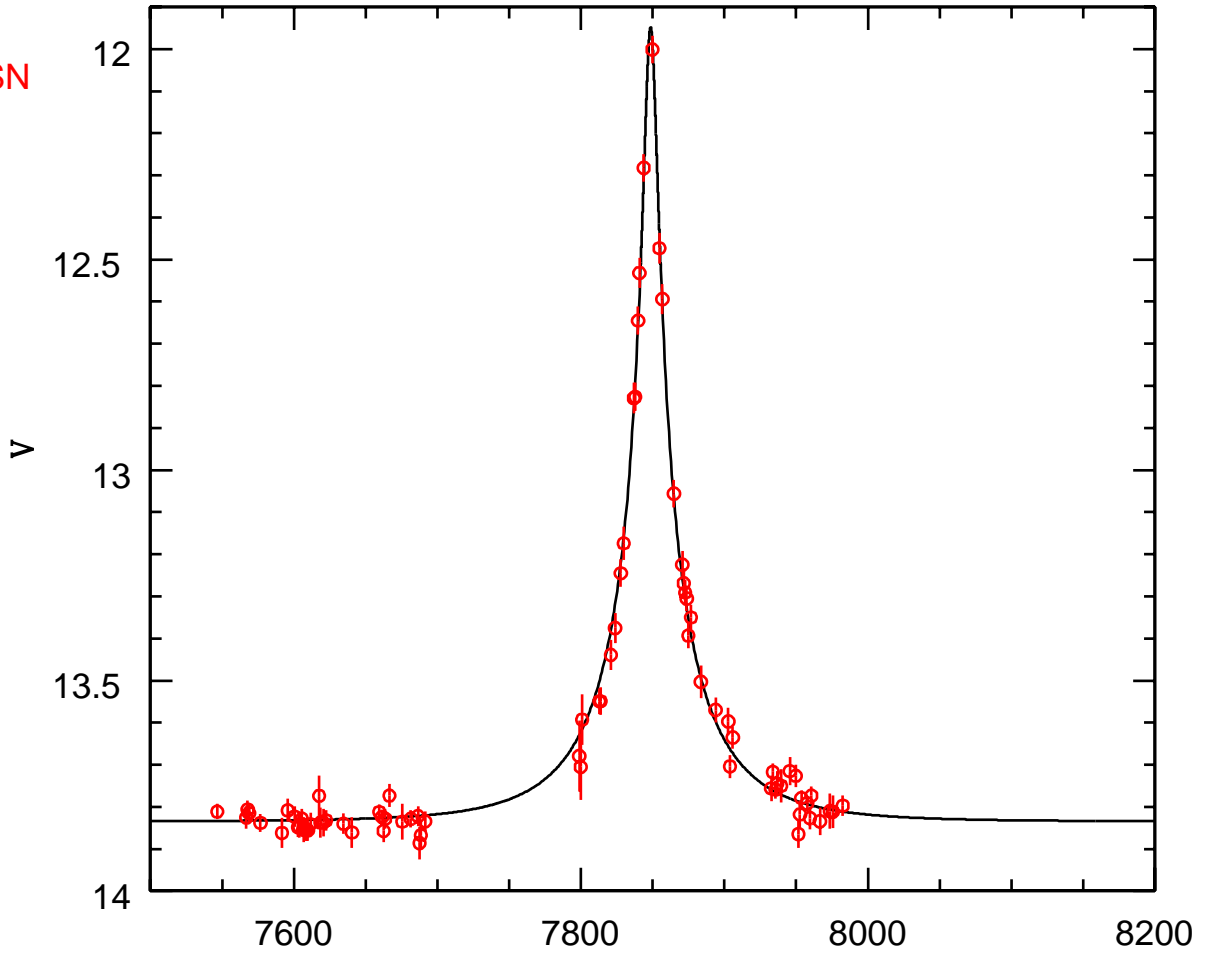
ASASSN-V J182456.34-305816.7
