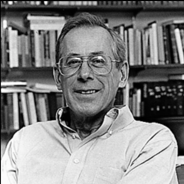
Jim Peebles
