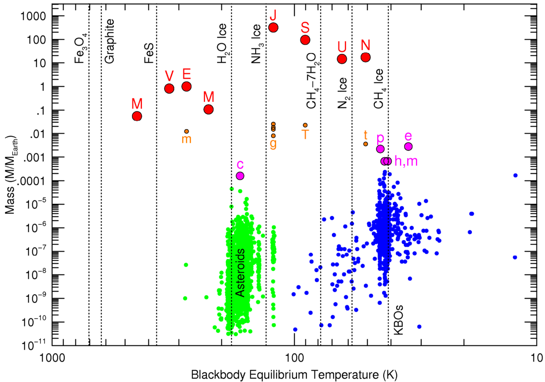
Condensation Temperatures from Lodders 2003, ApJ, 591, 1220
