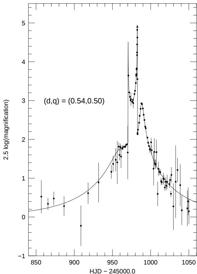
FIG. 3.—Predicted vs. “observed” deblened magnification for the close-binary model (d, q) = (0.54, 0.50) . The deblened magnification is A = (F - F_b)/F_s , where F is the observed flux and F_s and F_b are the fit source and background fluxes in the model. Data are binned, mostly in 1 day bins. However, for HJD' < 950 there are 10 day bins, and in the immediate neighborhood of the caustics there are 0.1 day bins. Data from all 14 light curves from the five collaborations are averaged together whenever they lie sufficiently close to fit in the same bin.
