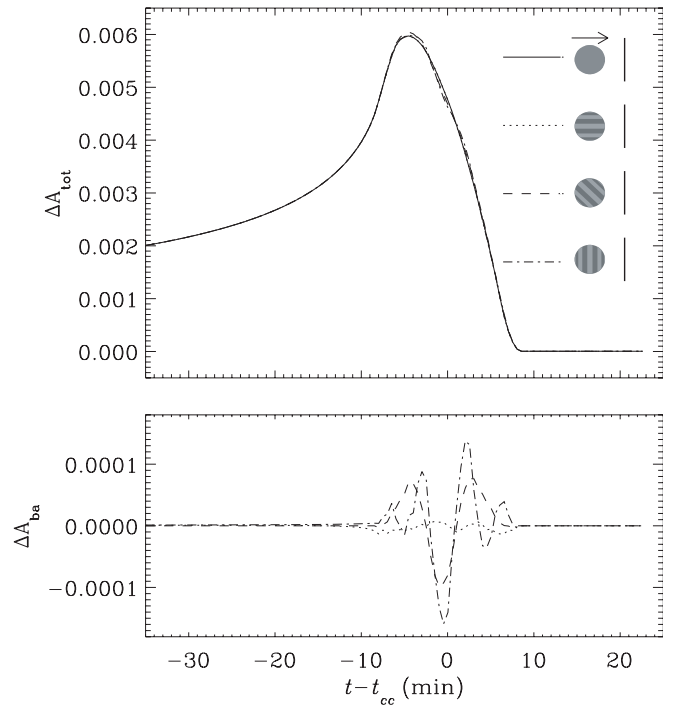
FIG. 9.— Top : Caustic-crossing microlensing light curves from a planet with and without zonal bands. The zonal bands are parallel with the planet's equator and cause alternate variations of the surface brightness, and the inclination of the planet is 90^\circ . The albedos of the bright and dark regions differ by 20%. The solid curve is the lensing light curve corresponding to a planet with uniform surface brightness. The lens system and the source trajectory responsible for the events are the same as for the light curves presented in Fig. 8. Bottom : Deviation \Delta A_{\text{ba}} caused by the zonal bands.
