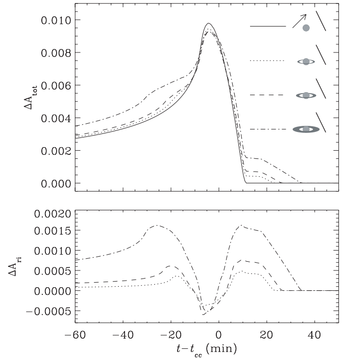
FIG. 4.— Top : Caustic-crossing microlensing light curves from a planet with inclined rings of different widths. The rings have a common inner radius of R_{\text{in}} = 2.0R_p but different outer ring radii of R_{\text{out}} = 2.6R_p, 3.0R_p , and 4.0R_p . The ring has an inclination of i = 75^\circ and albedo relative to the planet of 15%. The lens system and the source trajectory responsible for the events are the same as for the light curves presented in Fig. 2. Bottom : Additional magnification \Delta A_{\text{ri}} caused by the ring alone.
