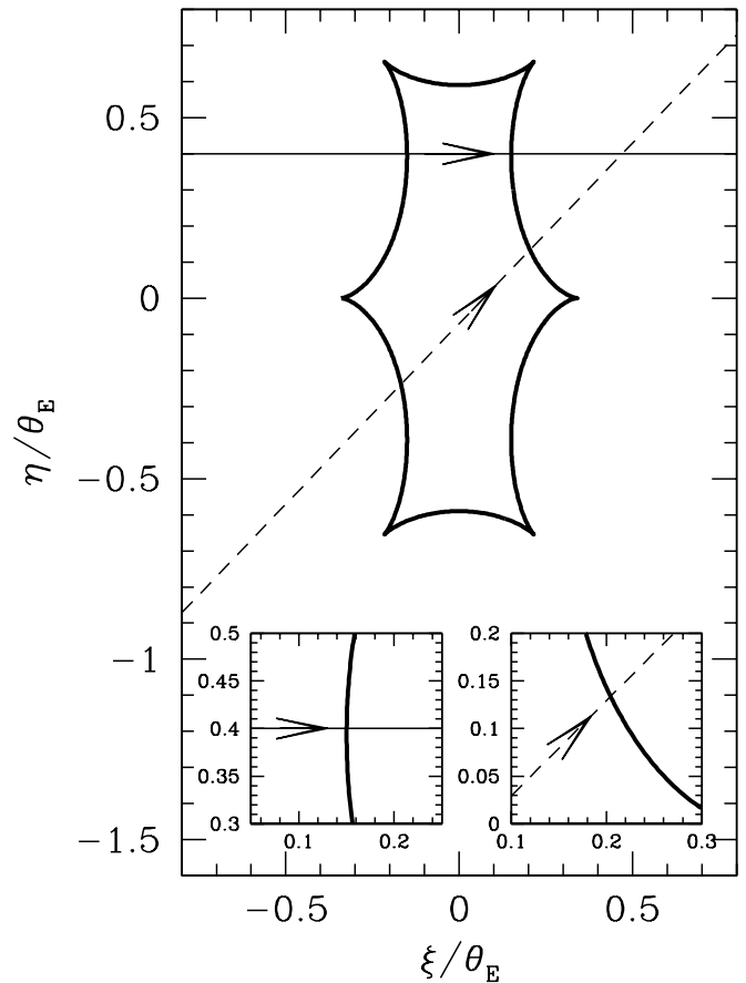
FIG. 1.—Example of the caustic structure ( thick solid curve ) produced by a binary lens. In this case, the system has equal-mass components separated by one Einstein ring radius. The coordinates are centered at the midpoint of the binary, and all lengths are normalized by the Einstein ring radius. The solid and dashed straight lines are the two source trajectories considered in the numerical simulations. The insets are the details of the regions around the second caustic crossings of these trajectories.
