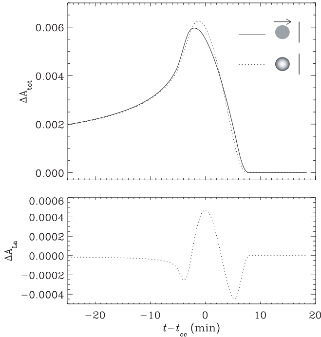
FIG. 10.— Top : Caustic-crossing microlensing light curves from a planet with the surface brightness profile expected from Lambert scattering (dotted line) and a uniform surface brightness profile (solid line). The lens system and the source trajectory responsible for the events are the same as for the light curves presented in Fig. 8. Bottom : Deviation \Delta A_{La} in the magnification of a Lambert sphere from a source with uniform surface brightness.
