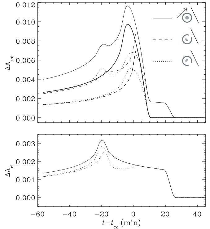
FIG. 6.— Top : Caustic-crossing microlensing light curves from a planet with a ring, where the planet's shadow is cast on the ring. Note that, because of the specific geometry of the planet, host star, and observer, the planet is at quarter-phase. Each ring has inner and outer ring radii of (R_{\text{in}}, R_{\text{out}}) = (2.4, 3.0)R_p , is seen face-on, and has an albedo relative to the planet of 15%. The lens system and the source trajectory responsible for the events are the same as for the light curves presented in Fig. 2. For all line types, the heavier curve is for the planet only, while the lighter curve is for the planet and the ring. Bottom : Additional magnification \Delta A_{\text{ri}} caused by the ring alone.
