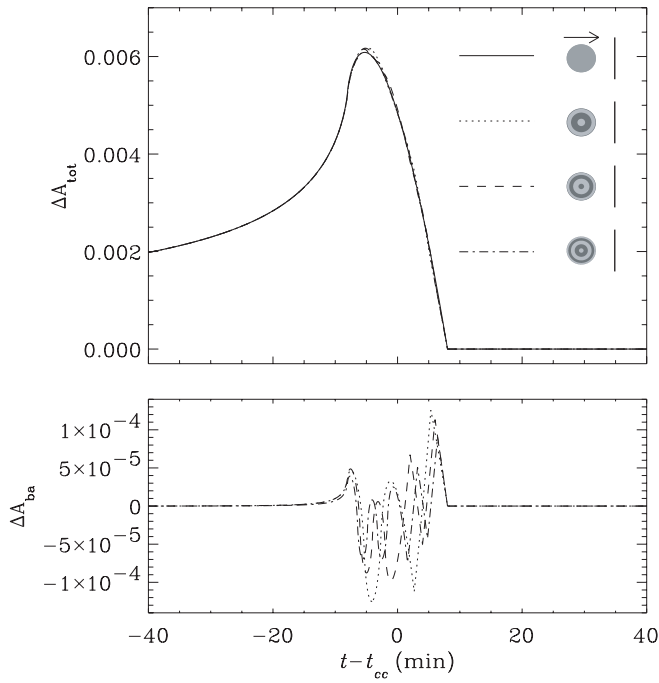
FIG. 8.— Top : Caustic-crossing microlensing light curves from a planet with and without surface albedo variations caused by zonal bands. The zonal bands are parallel with the planet's equator and cause alternate variations of the surface brightness, and the planet is seen pole-on. The albedos of the bright and dark regions differ by 20%, and the mean surface brightness of each model has been adjusted in order to match that from the uniform planet. The events arise from the second caustic crossing of the solid source trajectory through the binary lens systems depicted in Fig. 1. Bottom : Deviation \Delta A_{\text{ba}} caused by the zonal bands.
