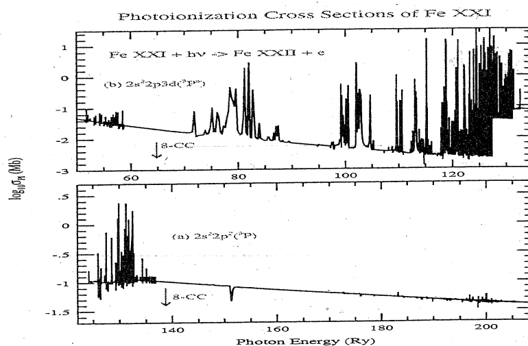
Figure 1. Photoionization cross-sections, \sigma_{PI} , of ground 2s^2 2p^2(^3P) and excited 2s^2 2p 3d(^3P^o) states of Fe XXI (Nahar 2002).
