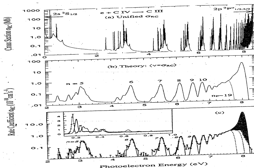
Figure 4. Comparison of theoretical and experimental recombination rate of C III (Pradhan et al. 2001).
