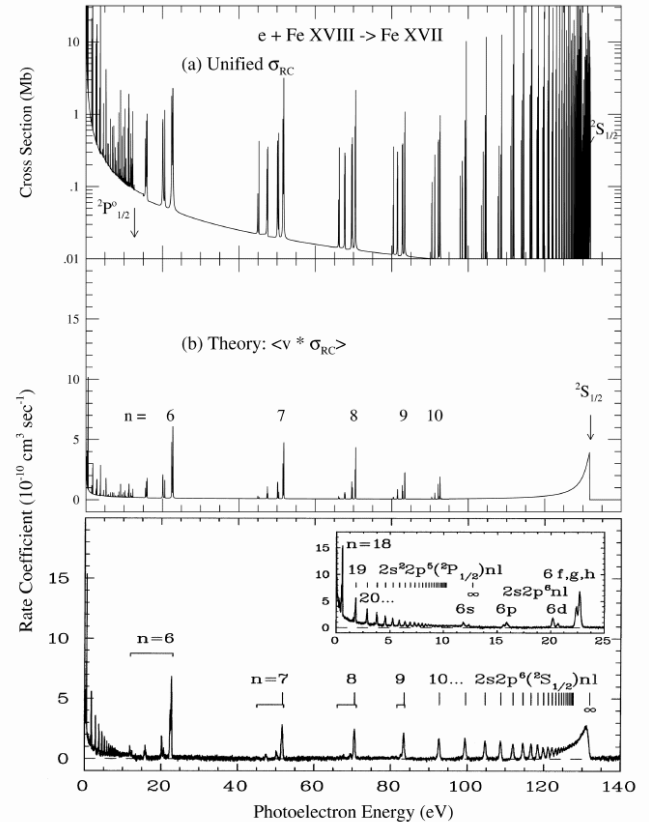
FIG. 1.—Unified recombination cross section \sigma_{\text{RC}} for Fe xvii. (a) Narrow Rydberg resonances converging to the 2s^2 2p^6 ({}^2P_{1/2}^o) threshold at 12.7 eV and the n -complexes belonging to the 2s 2p^6 ({}^2S_{1/2}) threshold are delineated. The high- n DR resonances are shown in the region E > 90 eV. (b) Theoretical rate coefficients ( \langle v \sigma_{\text{RC}} \rangle ) convolved over a Gaussian beam shape, compared to experimental data in the lower panel (Savin et al. 1999). The averaged theoretical DR contribution for resonances with 10 < \nu \leq \infty below the {}^2S_{1/2} threshold is analytically computed exactly.
