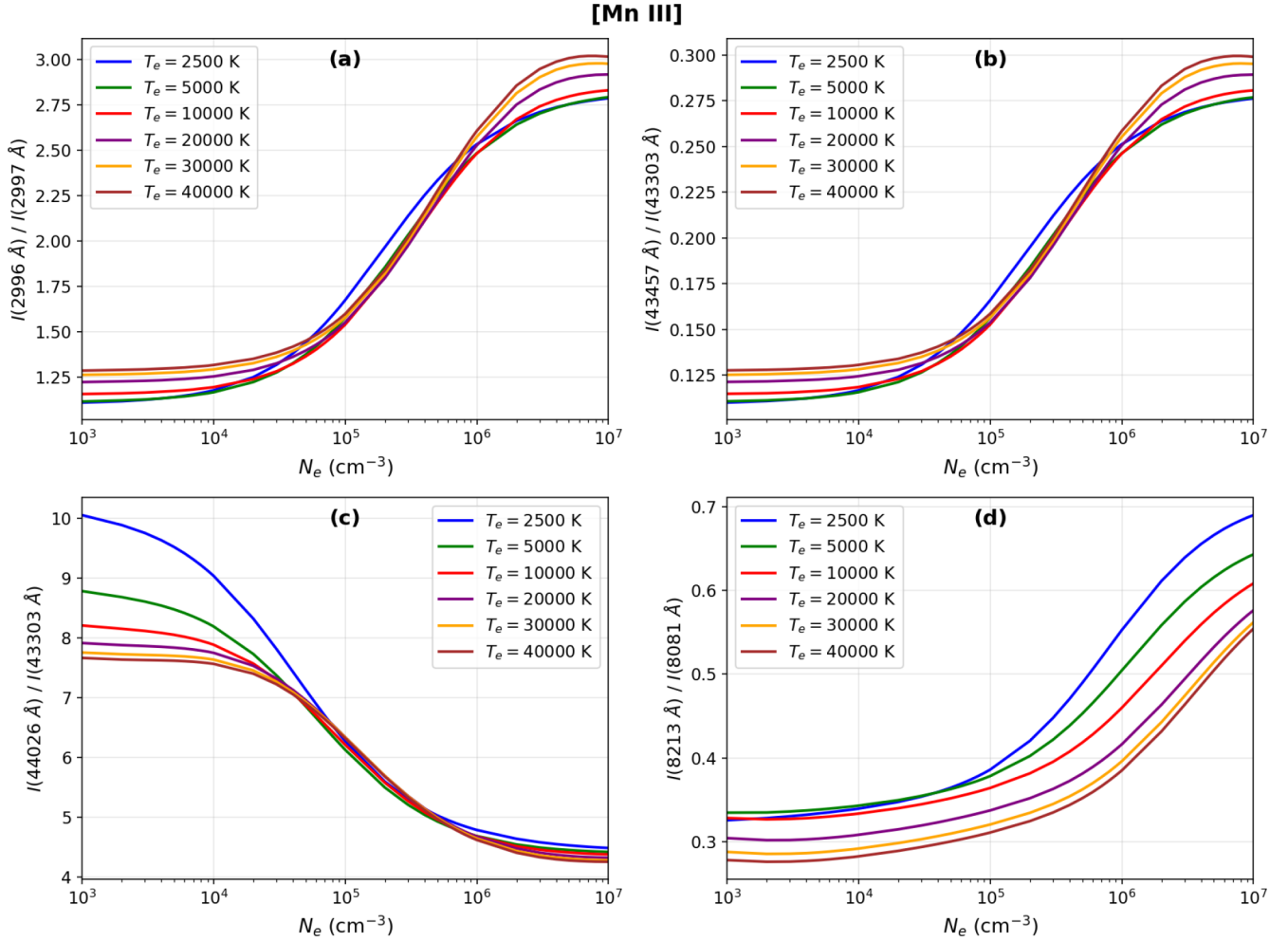
Figure 2. Mn III forbidden-line emissivity ratios as functions of \log_{10}(N_e/\text{cm}^{-3}) , at T_e = 2500, 5000, 10000, 20000, 30000 , and 40000 K. Top row: ratios nearly independent of T_e : (a) R_1: I(2996.42 \text{ \AA})/I(2997.45 \text{ \AA}), {}^4D_{5/2} \rightarrow {}^6S_{5/2} / {}^4D_{3/2} \rightarrow {}^6S_{5/2} . (b) R_2: I(4.35 \text{ }\mu\text{m})/I(4.33 \text{ }\mu\text{m}), {}^4D_{5/2} \rightarrow {}^4P_{3/2} / {}^4D_{3/2} \rightarrow {}^4P_{3/2} . Bottom row: ratios sensitive to both N_e and T_e : (c) R_3: I(4.40 \text{ }\mu\text{m})/I(4.33 \text{ }\mu\text{m}), {}^4D_{7/2} \rightarrow {}^4P_{5/2} / {}^4D_{3/2} \rightarrow {}^4P_{5/2} . (d) R_4: I(8213.52 \text{ \AA})/I(8081.28 \text{ \AA}), {}^2F_{5/2} \rightarrow {}^4P_{3/2} / {}^2D_{3/2} \rightarrow {}^4P_{3/2} .
