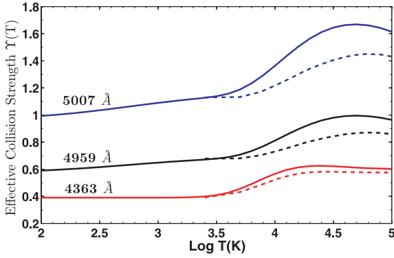
Figure 5. Effective collision strengths of the [O III] optical transitions ^1D_2\text{--}^3P_1 , ^1D_2\text{--}^3P_2 and ^1S_0\text{--}^1D_2 at \lambda\lambda 4959 , 5007 and 4363 , respectively (cf. Fig. 4).
