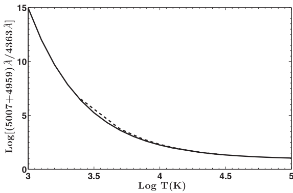
Figure 6. Blended [O III] line ratio (4959 + 5007)/4363 versus temperature, at N_e = 10^3 \text{ cm}^{-3} . The dashed line using earlier data (Aggarwal & Keenan 1999) is plotted down to 2500 \text{ K} .
