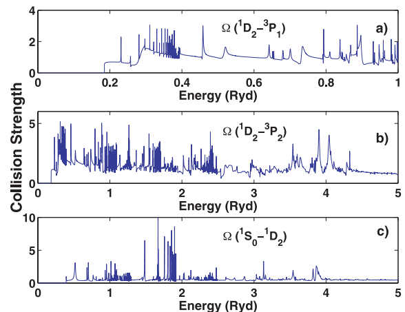
Figure 4. Collision strengths of the [O III] optical transitions. The two transitions ^1D_2-^3P_1, ^1D_2-^3P_2 in (a) and (b) have similar resonance structures; the top panel (a) presents an expanded view below E \leq 1 Rydberg.
