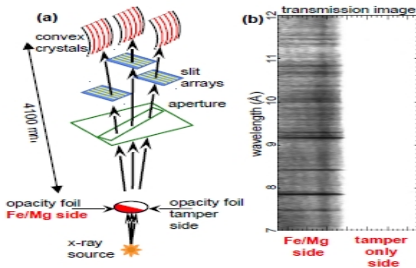
Fig. 5. Experiment. a: spectrometers view the half-moon shaped tamped iron/magnesium sample. Each spectrometer employs multiple slits to project space-resolved images onto a convex crystal that disperses the spectrum before recording on film. The setup measures the unattenuated (tamper only) and the attenuated (tamper plus FeMg) spectra on the same experiment. b: A space and spectrally-resolved transmission image is obtained by dividing the attenuated spectral image by the unattenuated image. Darker regions correspond to higher absorption. The white portion of the image corresponds to 100% transmission 1
