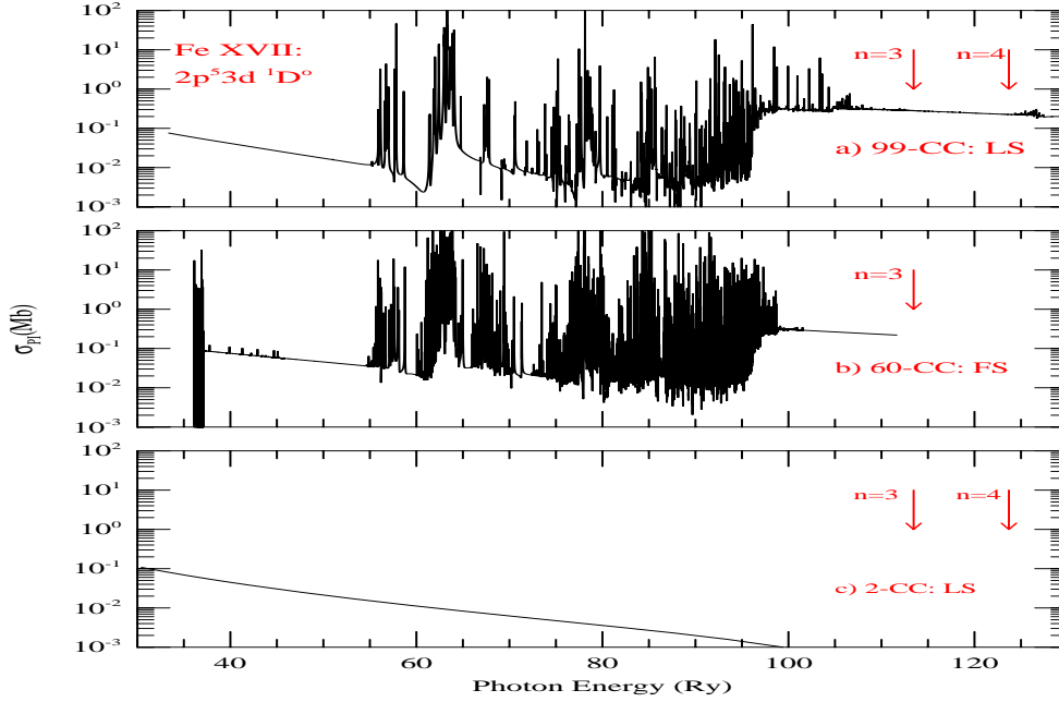
Fig. 9. Photoionization cross sections \sigma_{PI} of 2s^2 2p^5 3d(^1D^o) state of Fe XVII in the R-matrix calculations: a) present 99-CC expansion in LS coupling, b) 60-CC expansion in fine structure (FS), 8 c) 2-CC expansion in LS coupling under the OP. 14 The arrows indicate energy positions for the last n=3 and n=4 core excitations. \sigma_{PI} in FS (b) has more resonances due to couplings of more channels and finer energy mesh and in 99-CC LS (c) has additional resonances, although not very strong, and a very slow decaying background.
