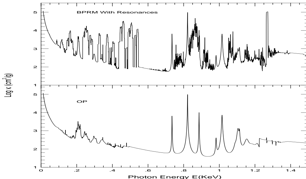
Fig. 8. Monochromatic opacity of Fe XVII at temperature T = 2.24 \times 10^6 K and electron density N_e = 10^{23} \text{ cm}^{-3} , corresponding to the base of the solar convection zone. The top panel presents opacity obtained using new atomic data from 60 CC wave function expansion and the bottom panel the total OP opacities which uses TOPbase data. 14 OP model includes resonances of high core-excitations, which are not included in the wave function expansion, as lines which are broadened with autoionization widths perturbatively, and the high-energy K-shell continuum opacity not yet included in 60-CC calculations 8
