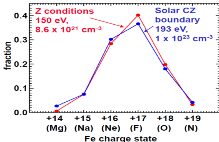
Fig. 4. Abundances of iron ions in the convection zone near the boundary with radiative zone in the sun as observed (blue) and measured (red).
