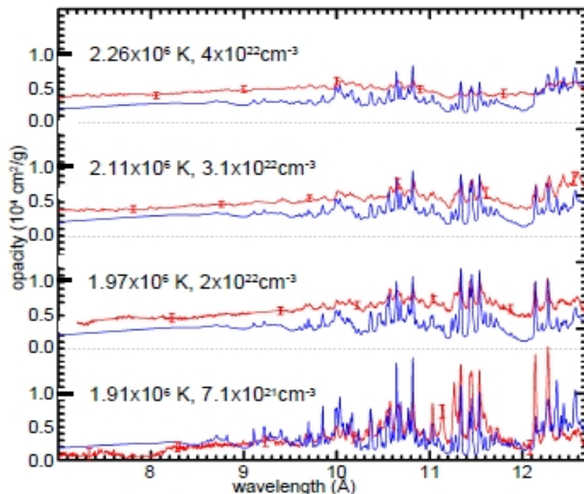
Fig. 6. Measured iron opacity spectra (red) at four T_e/n_e values are compared with predicted values (blue) calculated using the SCRAM model which accounts for the instrument resolution. With higher temperature and density the measured opacity becomes more featureless while the background shows larger difference with the predictions. 1
