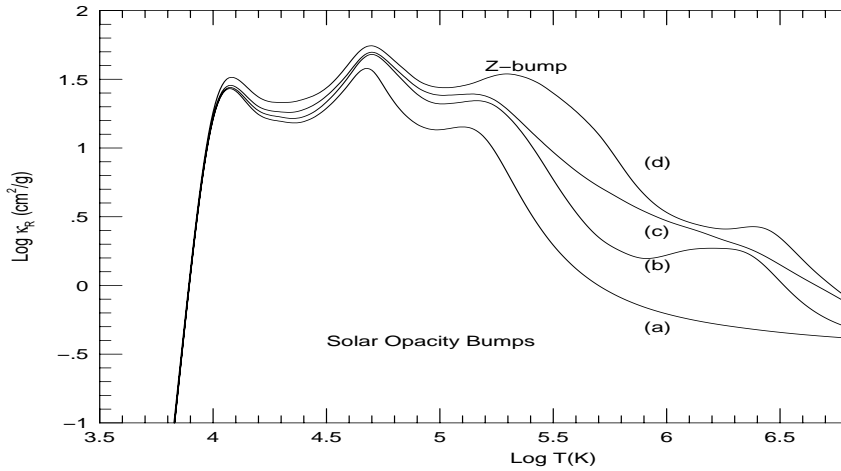
Fig. 3. Increment of Rosseland mean opacity \kappa_R with elements at R=3 . R = \rho(\text{g/cc})/T_6^3 , T_6 = T * 10^{-6} is related to depths in a star. Several bumps associated with excitation and or ionization of different atomic species are seen. The first (lowest \kappa_R ) curve (a) has three bumps corresponding to the ionization of neutral H, He, and He II, at \text{Log } T \approx 4, 4.6 , and 5.2 respectively. Including elements up to Ne raises the opacity towards higher temperatures as in curve (b). In addition, another bump appears at \text{Log } T \approx 6 - 6.5 which is related to highly ionized ions. Addition of further elements up to Ca raises the overall opacity significantly as shown in curve (c). The topmost curve (d) is due to the further inclusion of the iron group elements up to Ni, that gives rise to a considerable increase in opacity for all T > 10^4 K. The most outstanding enhancement in opacity due to iron occurs curve (d), \text{Log } T = 5.2 - 5.6 , referred to as the Z-bump. It is mainly due to excitation and ionization of Fe ions with partially filled M-shell ( n = 3 ), Fe IX - Fe XVI. 16
