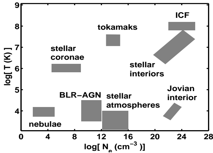
Fig. 1. plasma covers vast region in temperature-density ( T - \rho ) phase space and many physical regimes 6
