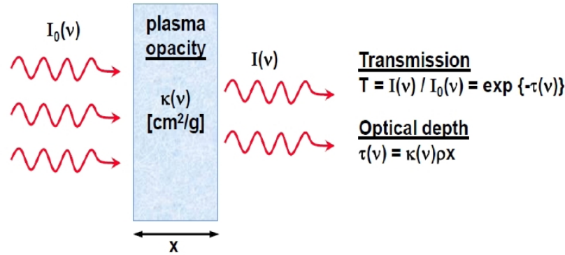
Fig. 2. Change in intensity of radiation passing through a distance of "x" in the plasma is due to the opacity.
