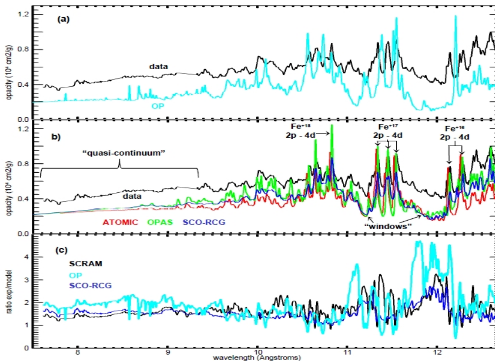
Fig. 7. Comparisons of observed iron opacity spectra (black curve) with multiple models. OP (cyan, at top and bottom panels), SCO-RCG (blue), ATOMIC (red), OPAS (light green) at the solar convection zone boundary temperature and density: T_e = 2.11\text{MK} , n_e = 3.1 \times 10^{22} \text{ cm}^{-3} . a. OP model uses for solar modeling. The dashed lines are the Rosseland mean opacities calculated for this wavelength range. b. Comparisons with three other models. c. Ratio of the experiment opacity with three different models. 1 Considerable differences can be seen between the measured and predicted opacities
