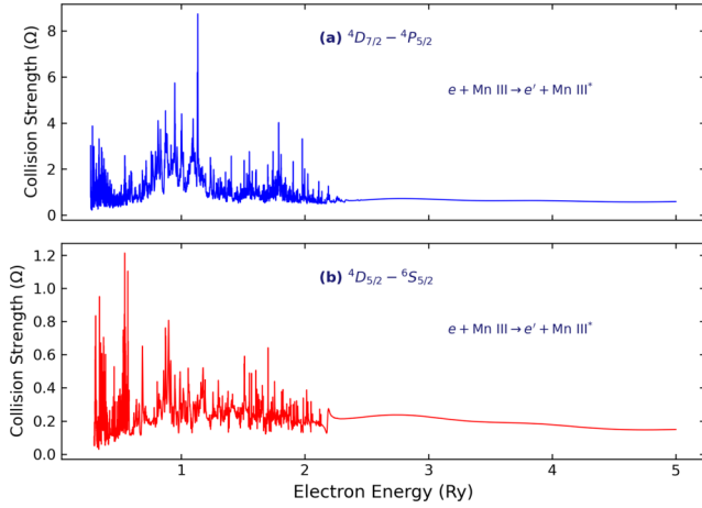
Figure 1. Collision strengths, \Omega , for the forbidden transitions (a) ^4D_{7/2} \rightarrow ^4P_{5/2} and (b) ^4D_{5/2} \rightarrow ^6S_{5/2} in Mn III as functions of electron energy (Ry). Prominent resonance structures are present in the near-threshold region, while smoother behaviour is observed at higher energies.
