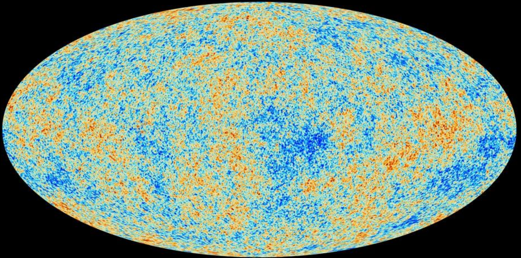
Planck CMB map
